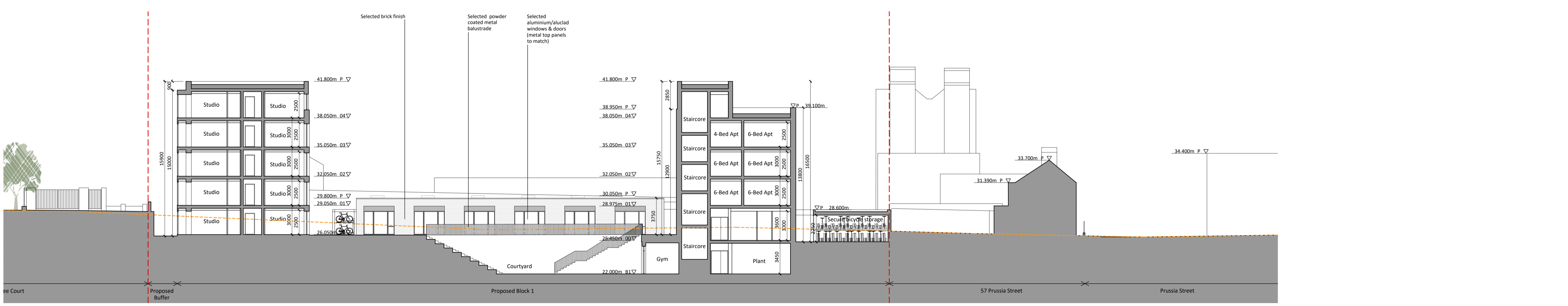
Section BB
